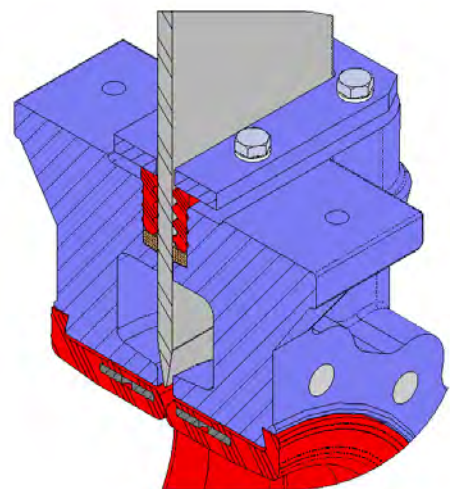
DETAIL C
