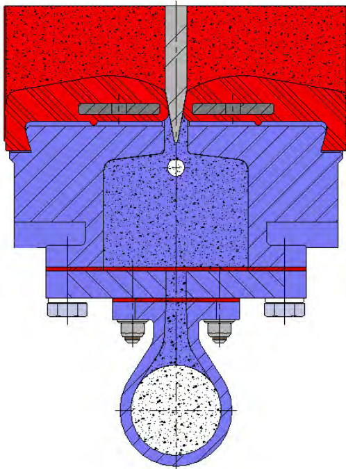
SECTION E-E
